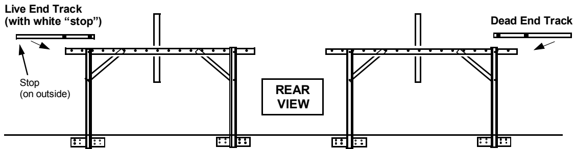
Double Base Frame—Models up 15 ft up to 24 ft
