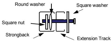
DETAIL—side view
